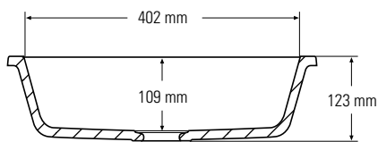
Side cross-section
